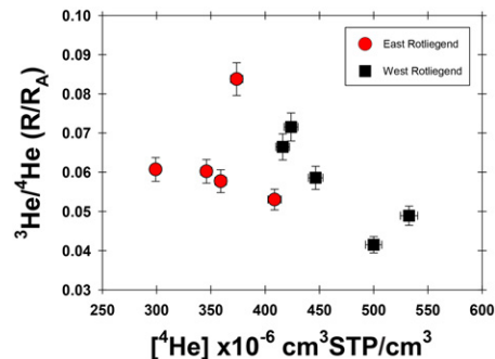
Figure 2. He isotopes ( 3 He/ 4 He) versus 4 He concentrations. STP—standard temperature and pressure conditions; R A = air 3 He/ 4 He.
