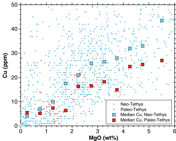
Figure 4. Cu versus MgO in Paleo-Tethyan and Neo-Tethyan igneous rocks; median values are used to highlight the data trends [sources of data: GEOROC database (Geochemistry of Rocks of the Oceans and Continents; http://georoc.mpch-mainz.gwdg.de ); Hess et al., 1995; Lemaire et al., 1997; Roger et al., 2003; Zhang et al., 2006a, 2006b, 2007; Cai et al., 2009, 2010; Dokuz et al., 2010; Karimpour et al., 2010; Yang et al., 2011, 2014; Mirnejad et al., 2013; de Sigoyer et al., 2014; Zhang et al., 2014; Xia et al., 2015; Zhang et al., 2016; Dai et al., 2017].
