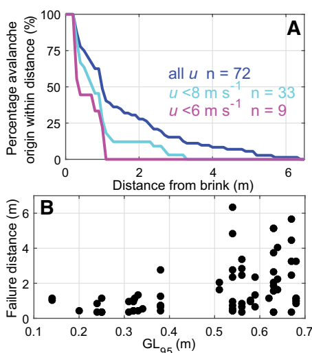
Figure 5. A: Cumulative frequency of detected point of avalanche origin with distance from the brink, including subsets of wind speeds ( u ) below 6 \text{ m s}^{-1} (magenta) and 8 \text{ m s}^{-1} (cyan). B: Distance from brink of avalanche initiation (failure distance) as a function of maximum grainfall length ( GL_{95} ).
