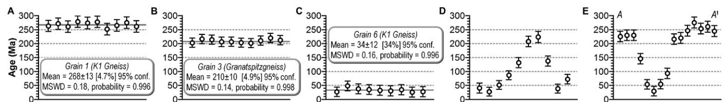
Figure 3. High spatial resolution chemical age profiles (step width 200–500 \mu\text{m} ) across single uraninite microcrystals. A–C: Homogeneous age distribution examples with calculated single grain ages of 268 \pm 13 , 210 \pm 10 , and 34 \pm 12 Ma, respectively. MSWD—mean square of weighted deviates; conf.—confidence. D, E: Polygenetic uraninite grains with heterogeneous age distributions (Granatspitz gneiss and Felbertauern augengneiss).
