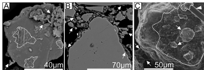
Figure 1. Backscattered electron and environmental scanning electron microscope (SEM) images of clay-coated grains. Arrows indicate clay coatings. Dashed lines outline the extent of the biofilm coats on the grain surface. A: SEM image of loose sediment. B: Thin section of clay-coated sand grains from an intertidal estuarine setting. C: Environmental SEM image of hydrated sediment. Triangle in top right points to a diatom with excreted extracellular polymeric substance grain attachment outlined.
