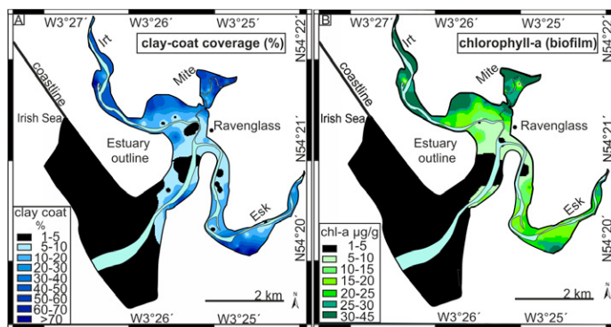
Figure 3. Maps of clay-coated sand grain distribution and biomarker proxy for tidal flat biofilm abundance on sand grains. A: Clay-coat coverage of sand grains established from quantitative petrography. Rivers Irt, Mite, and Esk are indicated. B: Chlorophyll-a concentrations. Darker shades in A and B represent greater extent of clay-coat coverage and greater abundance of sediment biofilm (chl-a—chlorophyll-a).
