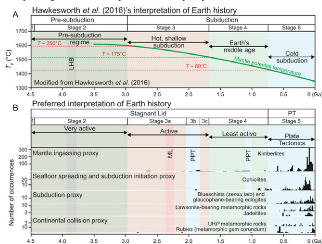
Figure 1. Alternate versions of Earth's tectonic evolution, both with subduction/plate tectonics, late, and pre-subduction/stagnant lid, early. A: The five stages of Hawkesworth et al. (2016). Stage 1—First few tens of millions of years: initial accretion and differentiation and magma ocean. Stage 2—Older than 3.0 Ga: generation of crust in a pre-plate tectonic regime. Stage 3—3.0–1.7 Ga: early plate tectonics—hot subduction with shallow slab breakoff. Stage 4—1.7–0.75 Ga: Earth's middle age, characterized by environmental, evolutionary, and lithospheric stability. Stage 5—younger than 0.75Ga: modern cold subduction. LHB—late heavy bombardment; PPT—proto plate tectonics; ML—magmatic lull of Condie et al., (2009). B: Our preferred alternate interpretation of Earth's tectonic history. Stage 1—First few tens of millions of years: initial accretion and differentiation and magma ocean. Stage 2—Older than 3.0 Ga: very active stagnant lid environment: many drips and plumes. Stage 3—3.0–1.7 Ga: active stagnant lid: fewer, larger drips and plumes, komatites and trondhjemite-tonalite-granodiorite intrusions during stage 3a, proto plate tectonics including ophiolites during stage 3b, abundant crustal production during stage 3c. Stage 4—1.7–0.75 Ga: least active stagnant lid: granites and anorthosites. Stage 5—younger than 0.75 Ga: sustained lithospheric subduction and true plate tectonics.
