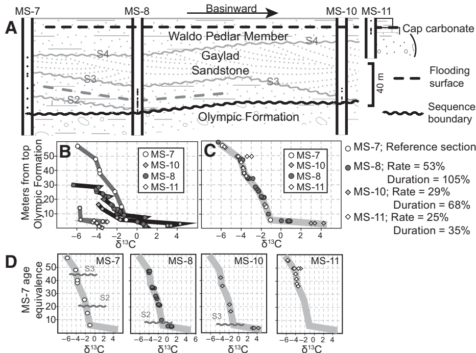
Figure 1. A: Sequence-stratigraphic relations among measured sections from the northeastern Amadeus Basin modified from Kennedy and Christie-Blick (2011); black dots are isotope samples from interfingered laminated cap carbonate facies. B: \delta^{13}\text{C} values relative to distance from top of Olympic Formation. C: \delta^{13}\text{C} values, accumulation rates, and net durations relative to reference section MS-7. D: temporal distributions of sequence boundaries if similar \delta^{13}\text{C} values are coeval (Fig. 1C).
