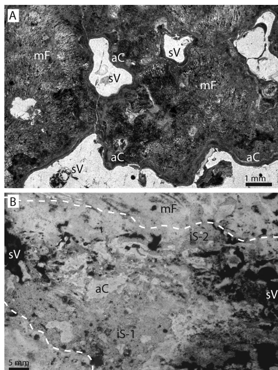
Figure 1. A: Example of partially cement-filled, irregularly shaped voids from a weakly laminated section of a modern microbialite at Lake Thetis, from Geological Survey of Western Australia Sample # F46287, Perth. B: Example of a void in a modern Bahamian microbialite partially filled with multiple generations of internal sediment and authigenic carbonate precipitates, from sample AC-1, stored at the Comparative Sedimentology Laboratory, Miami, Florida. aC—authigenic carbonate; iS—internal sediment; mF—microbial growth fabric; sv—secondary void; white line outlines filled void.
