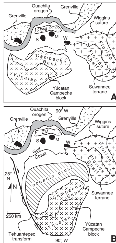
Figure 1. Pre-rift (A) and post-drift (B) configurations of the Gulf of Mexico region. EM—Eagle Mills rift basins. Uplifts (surface and subsurface): L—Llano; M—Monroe; S—Sabine; W—Wiggins.
