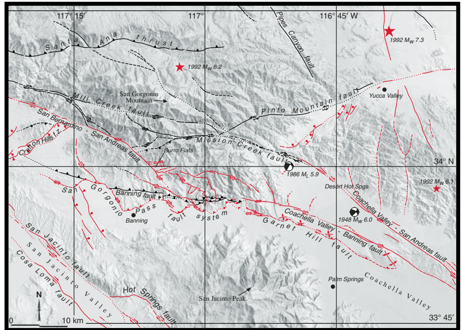
Figure 1. Shaded-relief topographic map of San Gorgonio Pass (SGP) region. Traces of active faults shown in red, inactive faults shown in black. Mapping from Allen (1957), Matti et al. (1985), and Yule and Sieh (2003). Beach-balls show epicenter and oblique slip during earthquakes on the north-dipping San Gorgonio Pass–Garnet Hill fault system at depth. Stars show epicenters of other earthquakes on faults outside of SGP.
