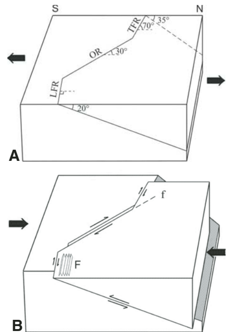
Figure 2. Simplified model showing two stages in the structural evolution of the Kangra recess. A: Geometry of initial fracture. LFR—leading frontal ramp; TFR—trailing frontal ramp; OR—oblique ramp; N-S—north and south directions. Note the variation of dip at the leading and trailing frontal ramps. B: Formation of folds (F), and extension of the oblique ramp fault (f) during the Himalayan orogeny.
