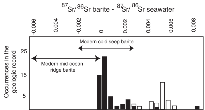
Figure 1. ^{87}\text{Sr}/^{86}\text{Sr} composition of barite expressed as difference from coeval seawater (redrawn from Maynard et al., 1995). Data differentiate barites originating in continental margin setting (black bars) from more radiogenic cratonic-type samples (white bars). Isotopic composition ranges of modern cold seep and oceanic ridge barite (Paytan et al., 2002) are also shown.
