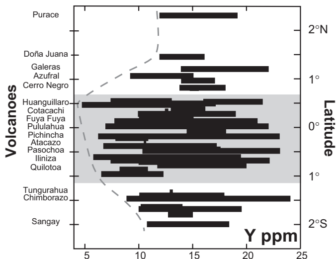
Figure 1. Variations in Y concentrations in Quaternary volcanic rocks of the Northern volcanic zone between 2.5°N and 2.5°S.
