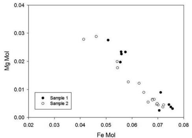
Fig. 8. Fe vs. Mg plot from EMPA showing homovalent substitution \text{Fe}^{2+} \rightarrow \text{Mg}^{2+} as indication of crystal zoning within perettiite-(Y). Mol corresponds to wt.% oxide/molecular weight; to obtain pfu (normalized to 2 Si apfu ) values have to be multiplied by 10.3.
