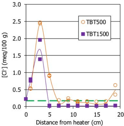
FIG. 6. \text{Cl}^- concentration in the aqueous extracts of samples of the two TH tests and of the original material (dashed line).
