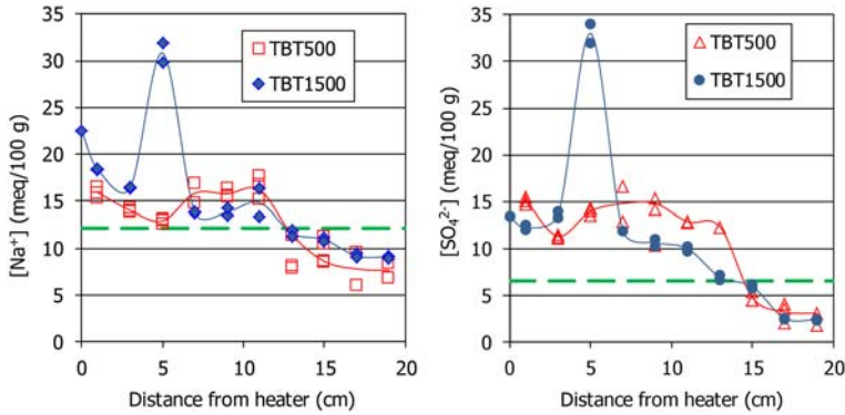
FIG. 5. Na and \text{SO}_4^{2-} concentrations in the aqueous extracts of samples of the two TH tests and of the original material (dashed lines).
