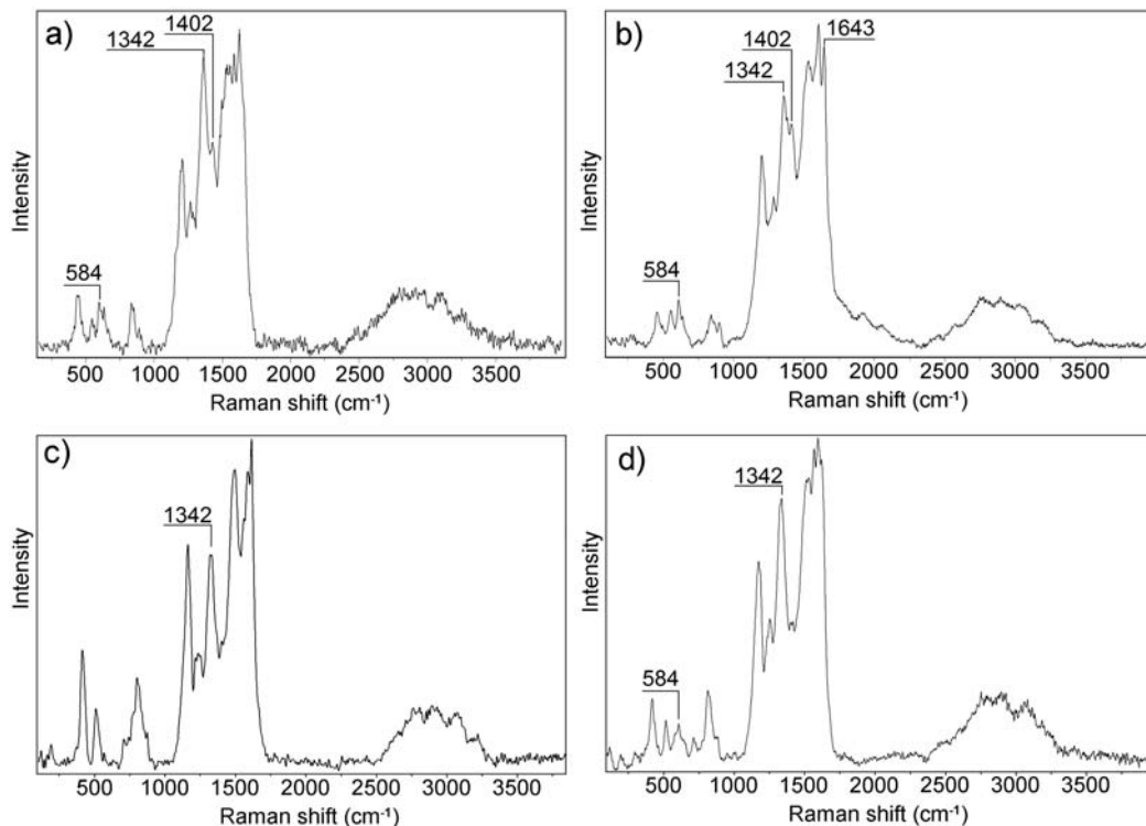
FIG. 7. Raman spectra: (a) of the PANI powder; (b) of the PANI/MMT powder; (c) of the PANI thin film; and (d) of the PANI/MMT thin film.
