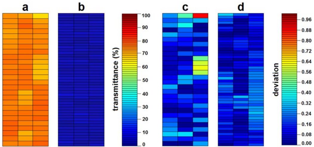
FIG. 10. Transmittance mapping across (a) the PANI and (b) the PANI/MMT thin films for wavelength \lambda = 520 nm, with deviations from the average values (c) for the PANI and (d) the PANI/MMT thin films. It is evident that rough surface of the pure PANI films is less homogeneous than the smooth surface of the PANI/MMT thin film.
