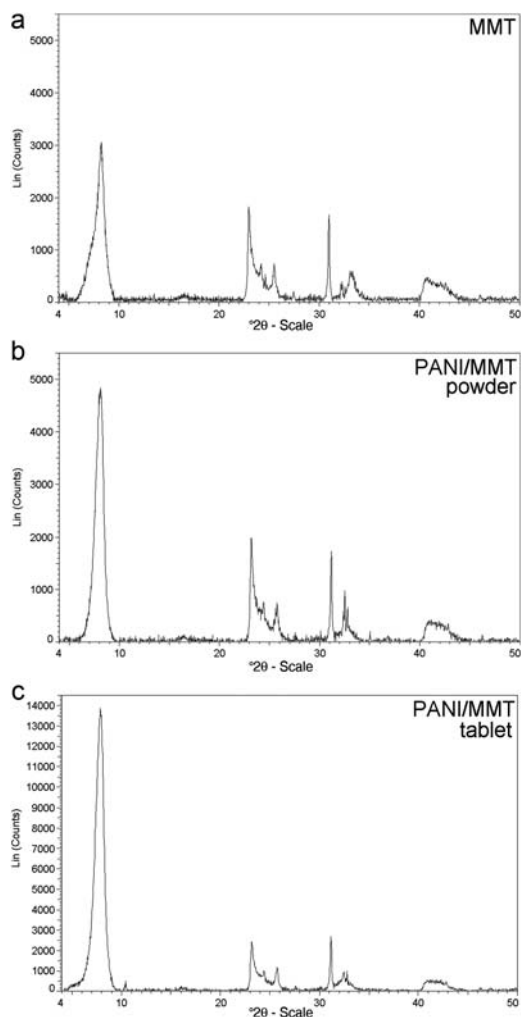
FIG. 4. Full diffraction patterns (range 4–50°2 \theta ) of the MMT powder, the PANI/MMT powder and the PANI/MMT pressed pellet.
