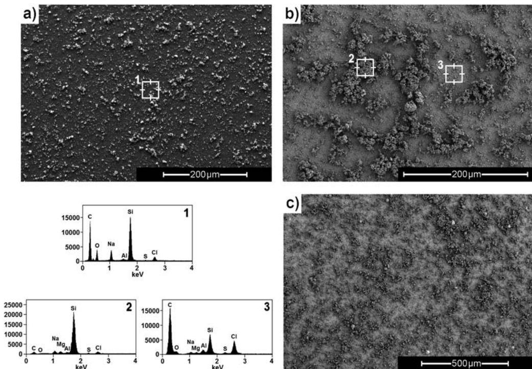
FIG. 11. SEM images (a–c) and EDX spectra at points 1–3 indicated on the PANI thin film (a, 1) and PANI/MMT thin film (b, 2 & 3 and c).
