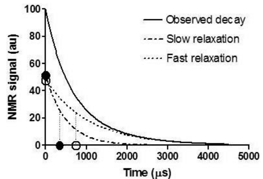
FIG. 3. Typical result from the NMR measurements on water-saturated MX-80 bentonite showing an observed decay curve (solid line), which could be split into two exponential functions (dotted lines), each one associated with a different relaxation time. The data points show zero time magnetization on the y axis and T_{1\rho} relaxation times on the x axis. Filled and open circles refer to fast and slow relaxation, respectively.
